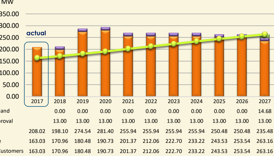
Supply-Demand Profile
