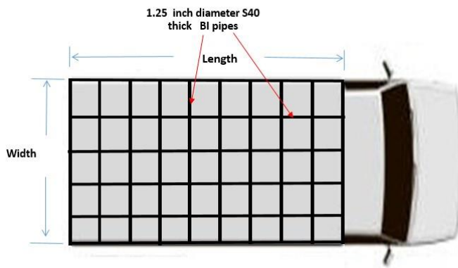
TOP VIEW( 6 Wheeler Truck ) LPG Hauler with OPEN CAGE
